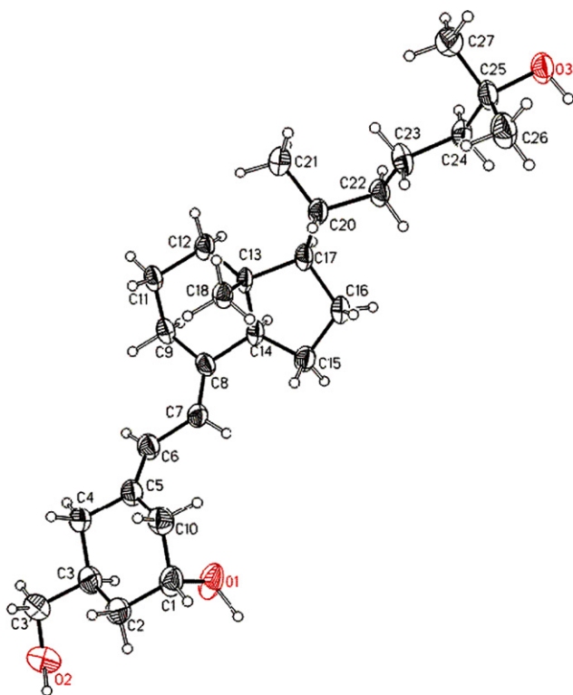
Figure 1. X-ray structure of 19-nor VD 3 analog 6b .
